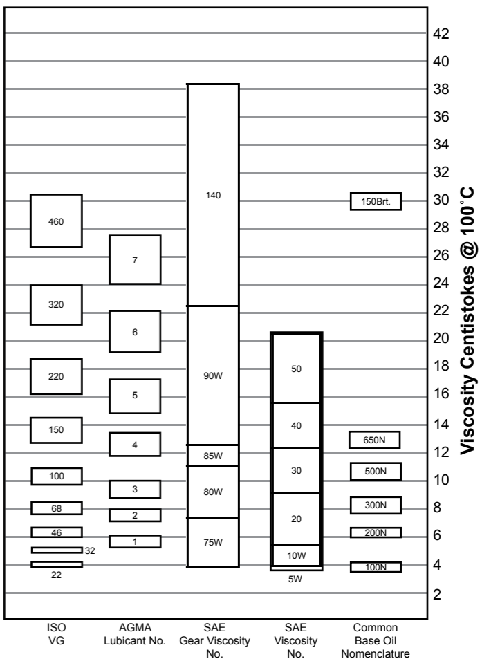
Comparative Oil Viscosity Classifications
